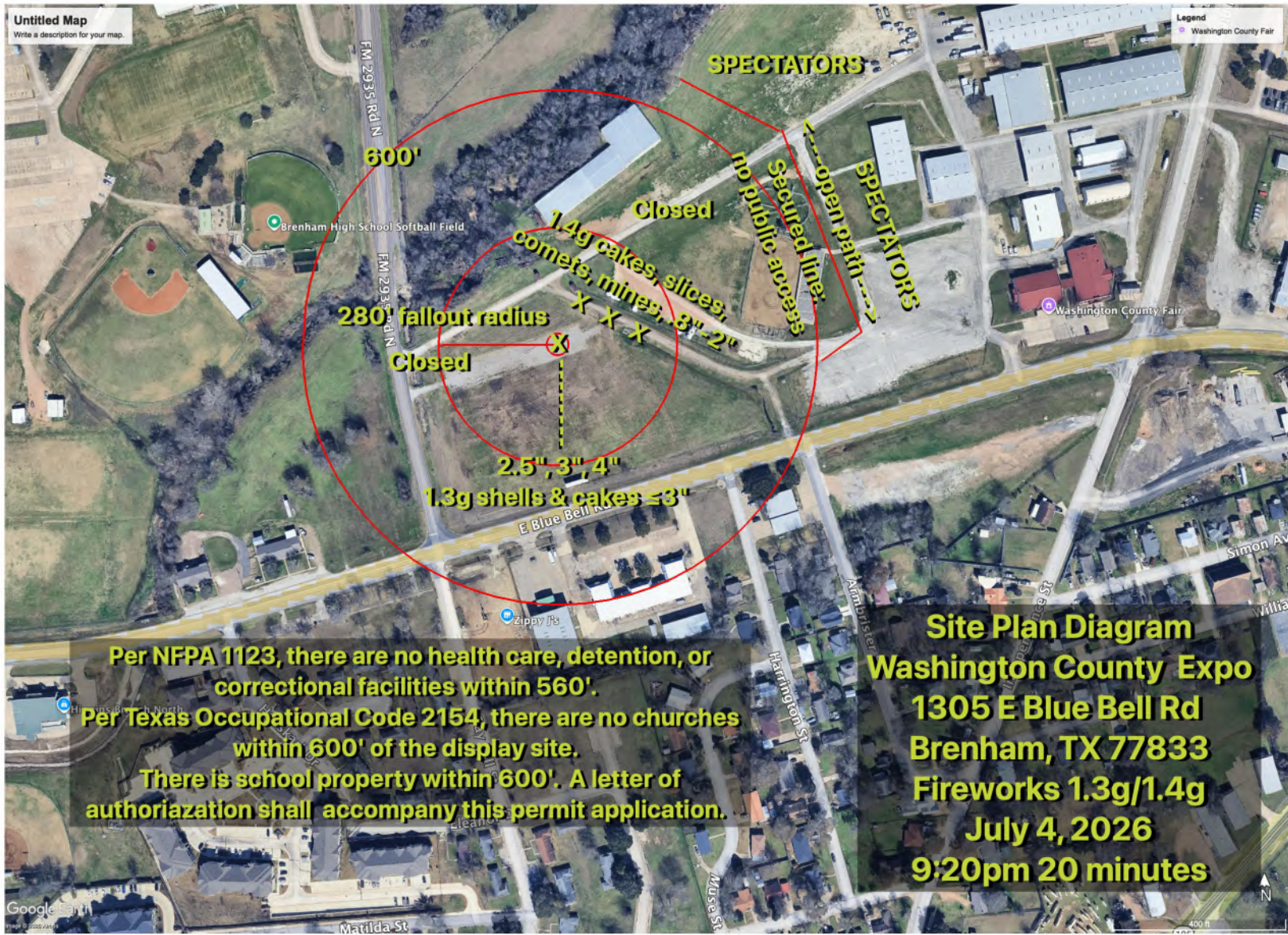
Figure 1 Site Plan Diagram
